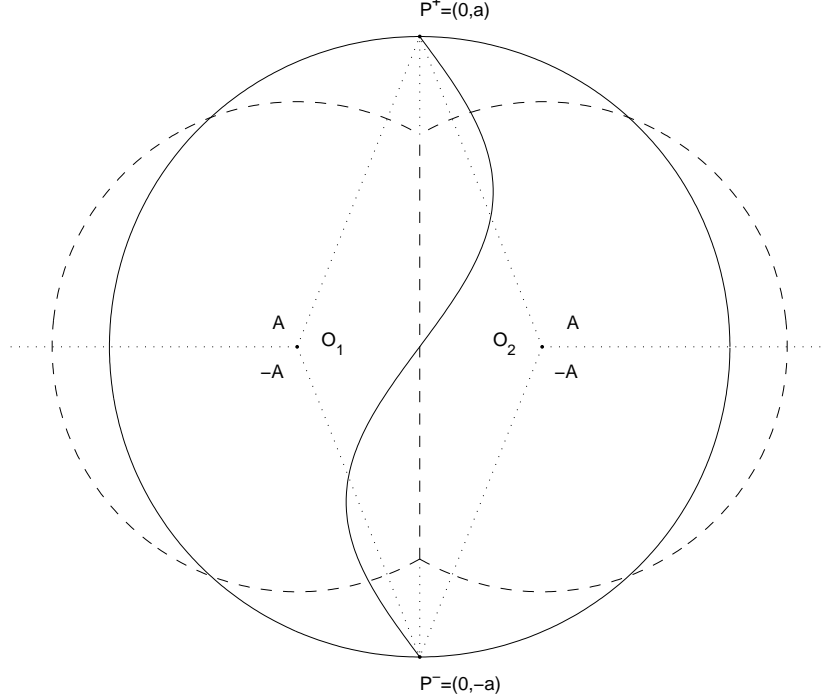
Figure 3: A standard double bubble is enclosed by the dashed curves in a (\xi, \theta) -frame; the solid curves bound a restrictedly perturbed double bubble; also plotted are the centers O_1 and O_2 , triple junction points P^+ and P^- , and the height a of P^+ and the angle A ; the triangles \triangle O_1 P^+ P^- and \triangle O_2 P^+ P^- are mentioned in section 6.
