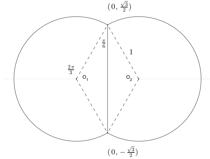
Figure 2: The equal area double bubble (E_1, E_2) where the radius of the two bubbles is 1. In each bubble the area of the sector is \frac{2\pi}{3} and the area of the triangle is \frac{\sqrt{3}}{4} .
