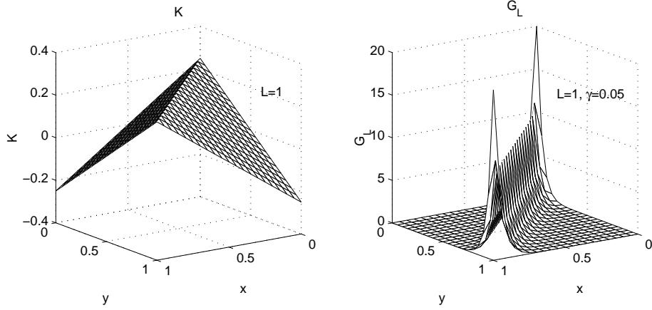
Figure 2: The kernels K(x, y) = \frac{L}{4} - \max\{x, y\} + \frac{1}{2}(x + y) and G_L(x, y) = \frac{1}{\gamma(e^{L/\gamma} - e^{-L/\gamma})} [\cosh(\frac{x+y-L}{\gamma}) + \cosh(\frac{|x-y|-L}{\gamma})] .
