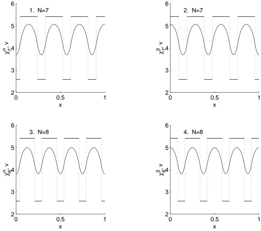
Figure 3: Metastable configurations with N = 7 and 8 . Shown are the graphs of \chi_N^{\alpha,\beta} and the corresponding v = (-\gamma^2 D^2 + 1)^{-1} \chi_N^{\alpha,\beta} . Here \alpha = 2.59 , \beta = 5.41 , d = 4.5 .
