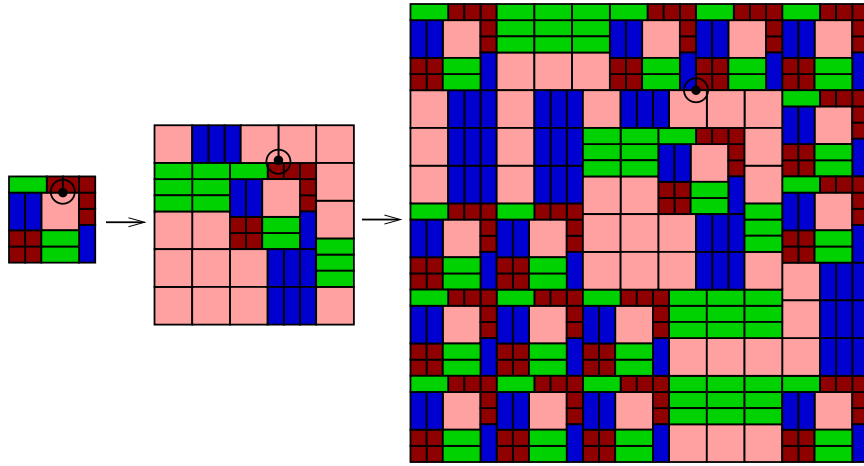
FIGURE 2. Three iterations of the larger square tile.
