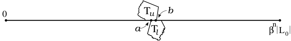
FIGURE 5. The simple adjacency \alpha is equivalent to T_u \cup T_\ell .
