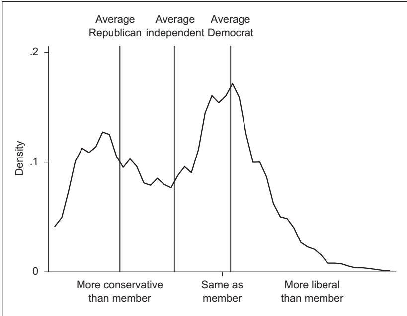
Figure 2. Constituent perceptions of ideological distance from Democratic incumbents
