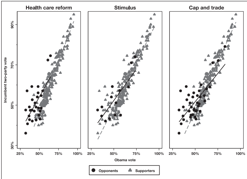
Figure 3. Roll call imbalance by district partisanship
