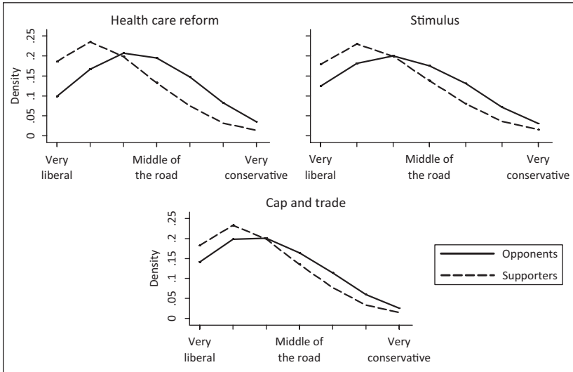
Figure 1. Constituent perceptions of ideologies of Democratic incumbents
