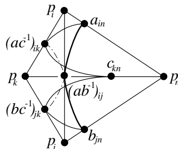
FIGURE 1. The sole nontrivial case when checking property (E3) of Theorem 2.1 for Dowling lattices.
