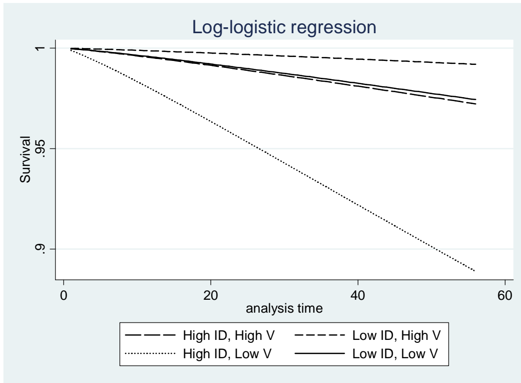
Figure 1: Survival Curves for High and Low Values of Ideological Distance and Vitality; from Log-Logistic, Shared Frailty Model
