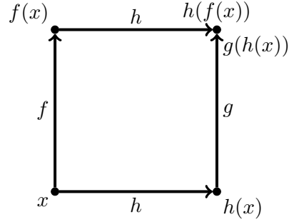
Figure 2.3: Commutative diagram for isomorphic (2,1):1 structures.
