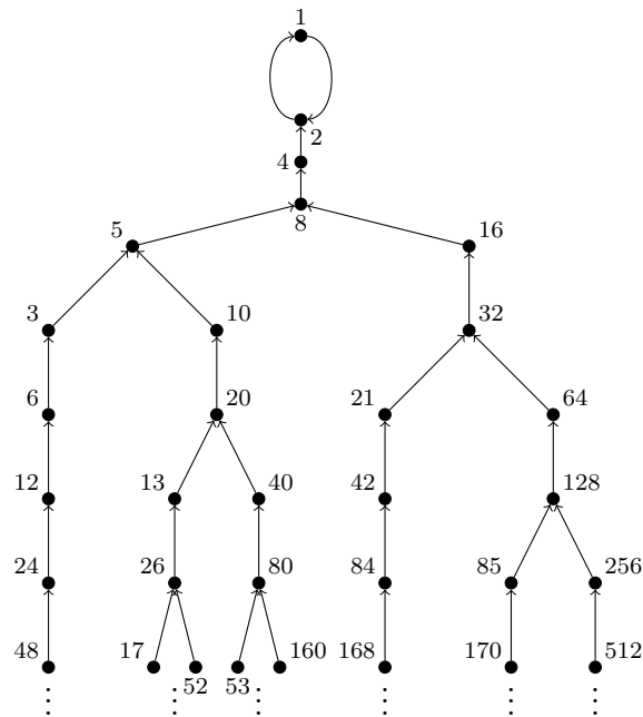
Figure 3.3: The Collatz graph.
