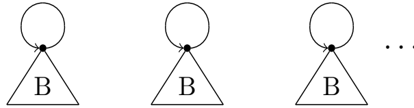
Figure 3.1: A computably categorical structure \mathcal{A} with infinitely many 1-cycles.
