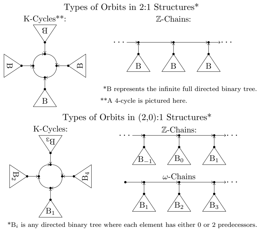
Figure 1.5: Types of orbits in two-to-one structures and (2,0):1 structures.
