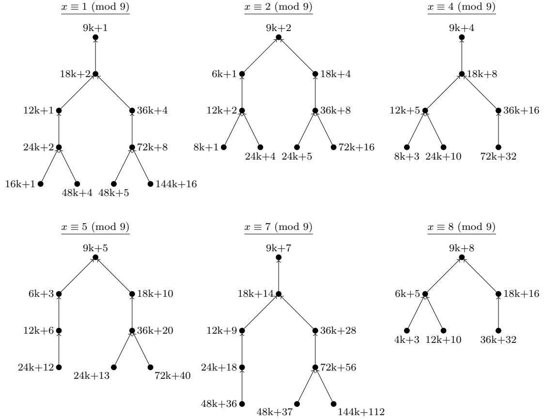
Figure 3.4: Truncated Trees for residue classes modulo 9 (where k > 0 ).
