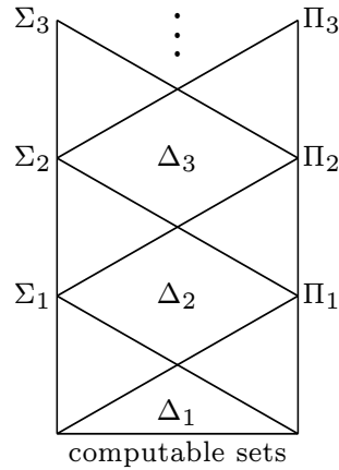
Figure 1.2: The arithmetical hierarchy.
