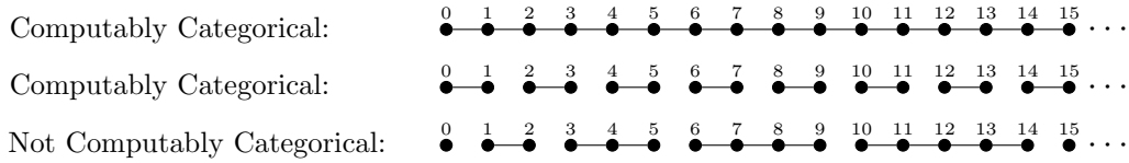
Figure 1.3: Computable graphs that are and are not computably categorical.
