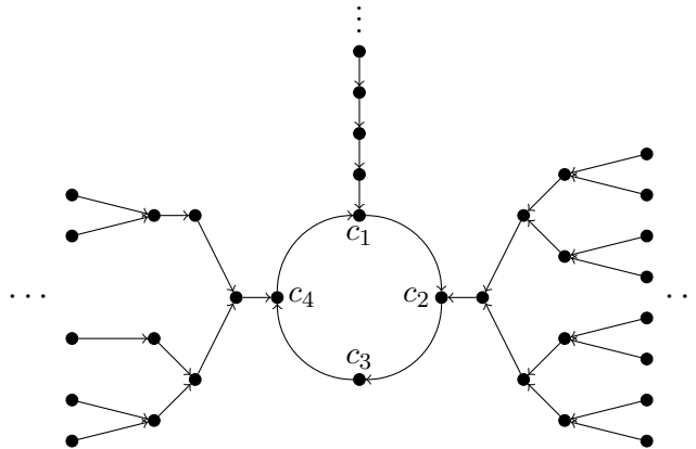
Figure 2.1: An example of a 4-cycle.
