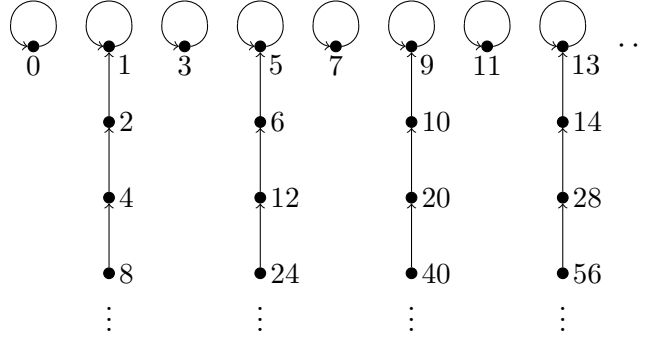
Figure 3.2: The directed graph of \mathcal{A} .
