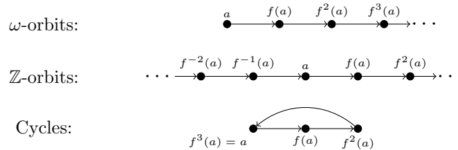
Figure 1.4: The three types of orbits in an injection structure.
