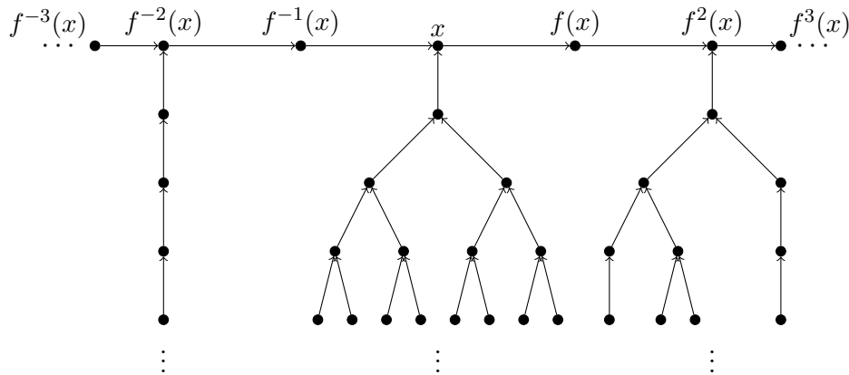
Figure 2.2: An example of a \mathbb{Z} -chain.
