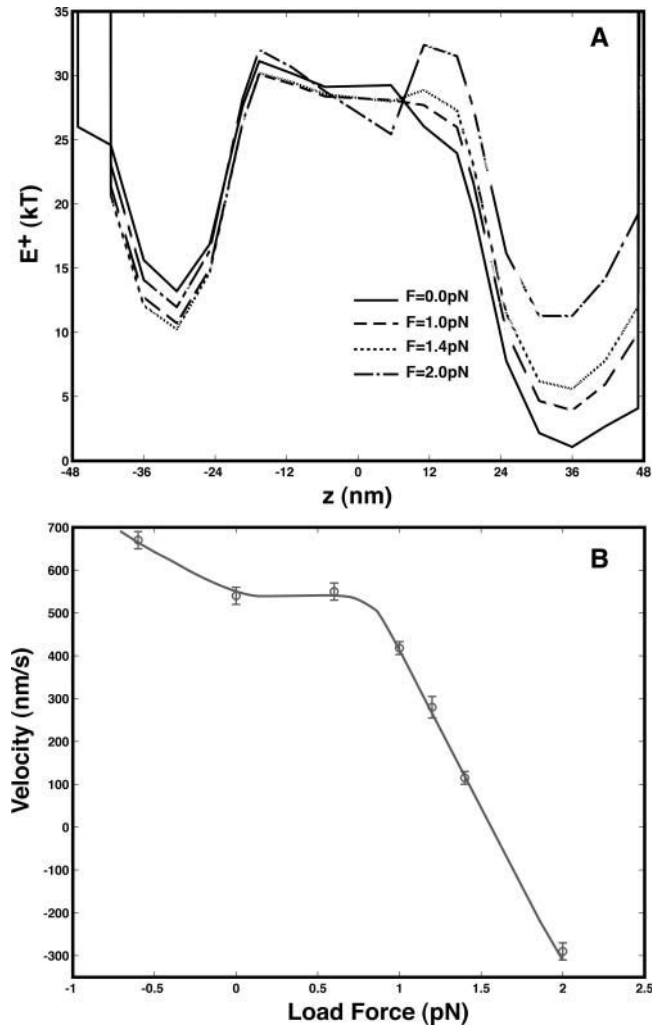
FIGURE 5 (A) The change in the transition state energy, E^\dagger(z) , for the leading head binding to actin. The value E^\dagger is a function of z and (\theta_1, \theta_2) . For this plot, (\theta_1, \theta_2) are chosen to be at the equilibrium position just before both heads are bound. The preferred binding location is always at 36 nm. The relative probability of binding to a different site is e^{-\beta(E^\dagger(z') - E^\dagger(z))} . (B) Force versus velocity curve for myosin-V. The symbols are from our Monte Carlo simulations. The line through the symbol is simply a guide for the eye. The predicted stall force is \sim 1.7 pN.
