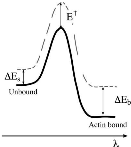
FIGURE 4 The transition state energy for binding to actin, E^\dagger , is determined by the elastic energy of the complex before ( \Delta E_s ) and after ( \Delta E_b ) binding.
